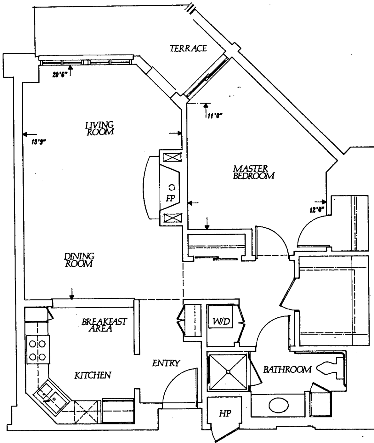
AVON FLOOR PLAN 880 SF
